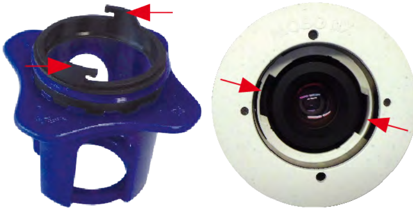
Fig. 36: Insert lens protection glass using the lens wrench
